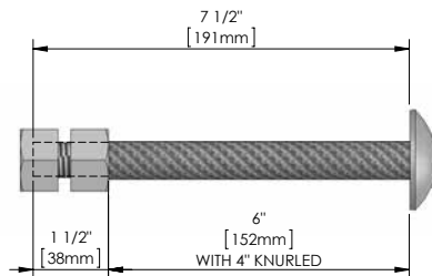
STANDARD STEP BOLT - 3/4\"/>
