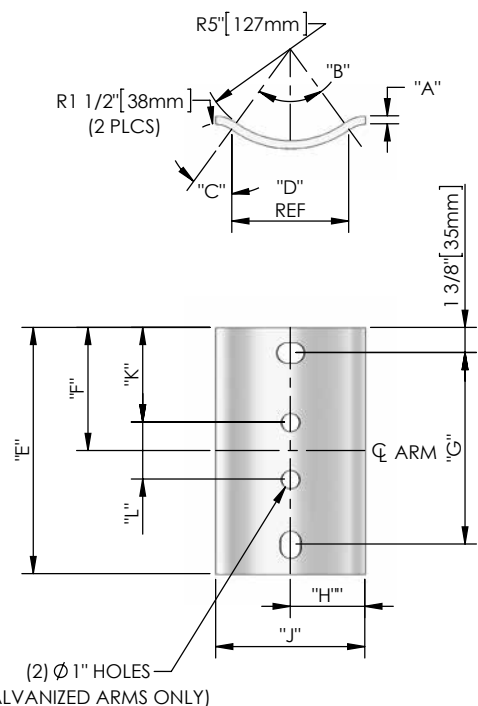
BRACKET 'A' STANDARD
