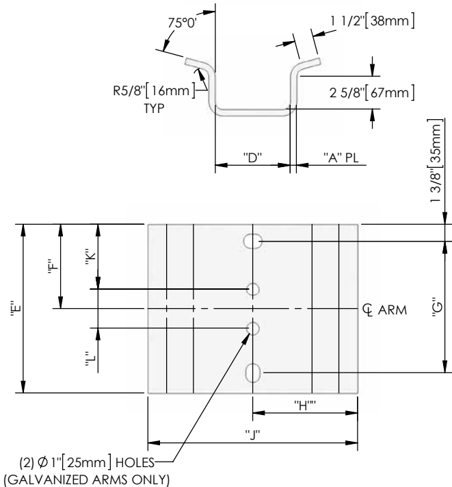
BRACKET 'C' ALLOWS INDEPENDENT MOUNTING OF TWO ARMS BACK TO BACK AT ONE ELEVATION.
